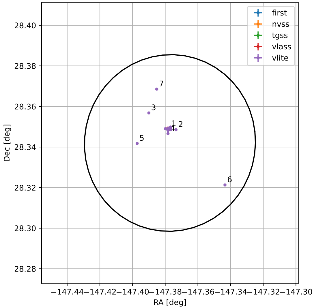
4FGL J1410.4+2820
