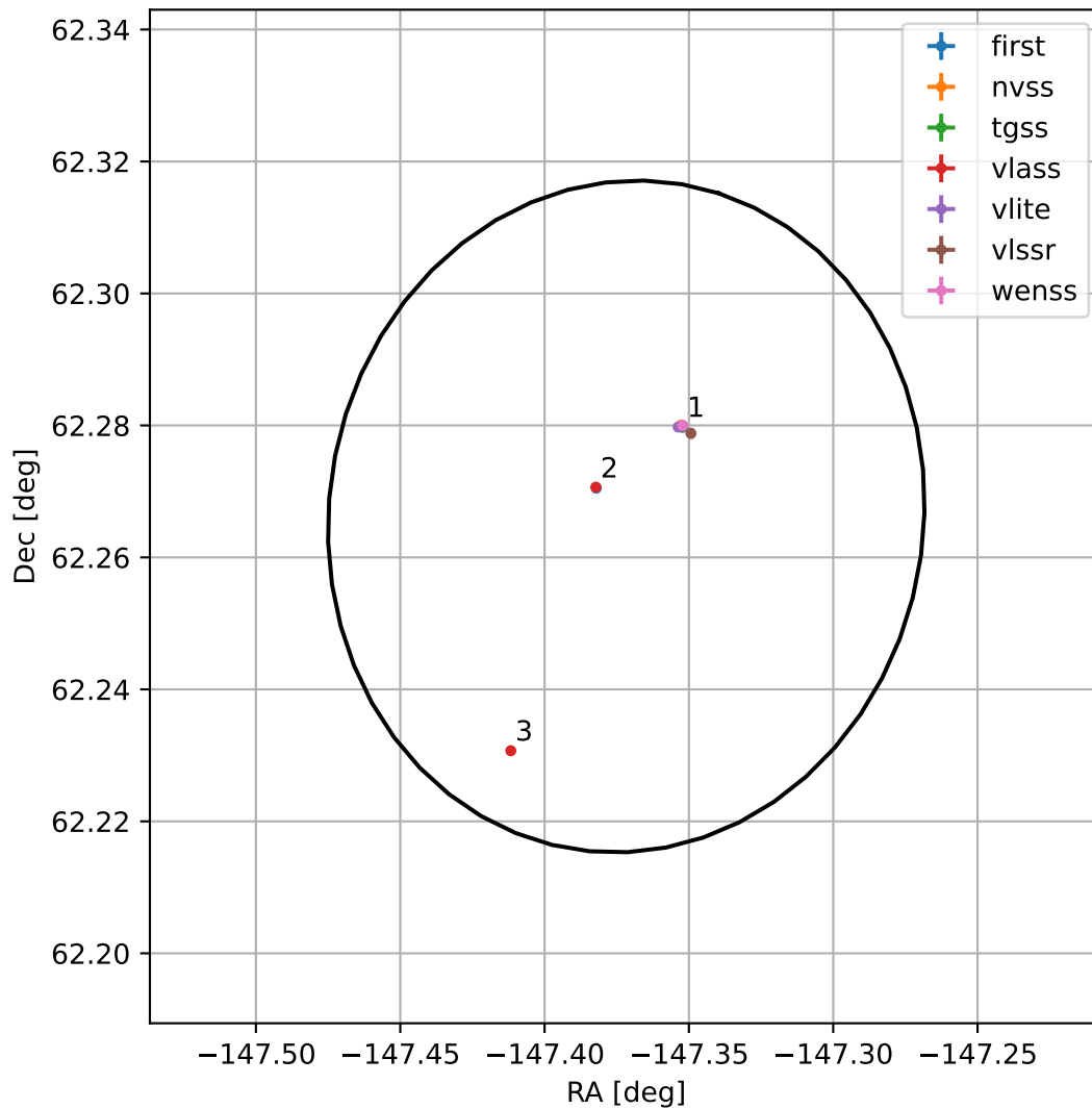
4FGL J1410.5+6215
