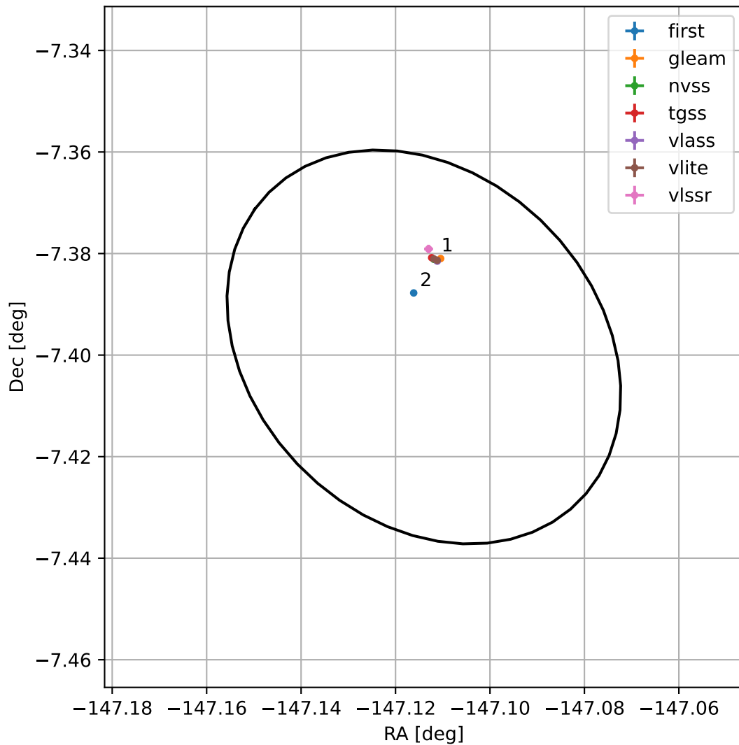
4FGL J1411.5-0723
