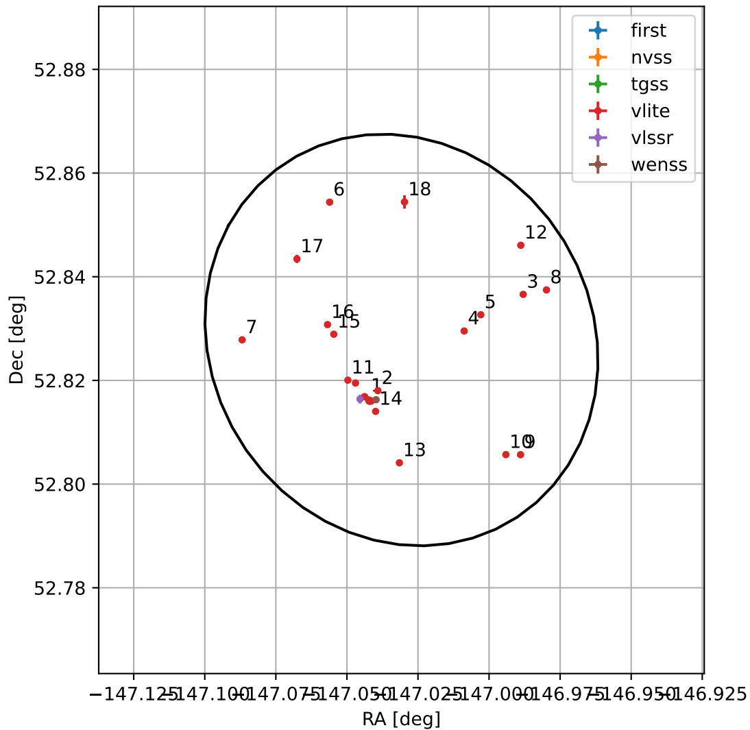
4FGL J1411.8+5249
