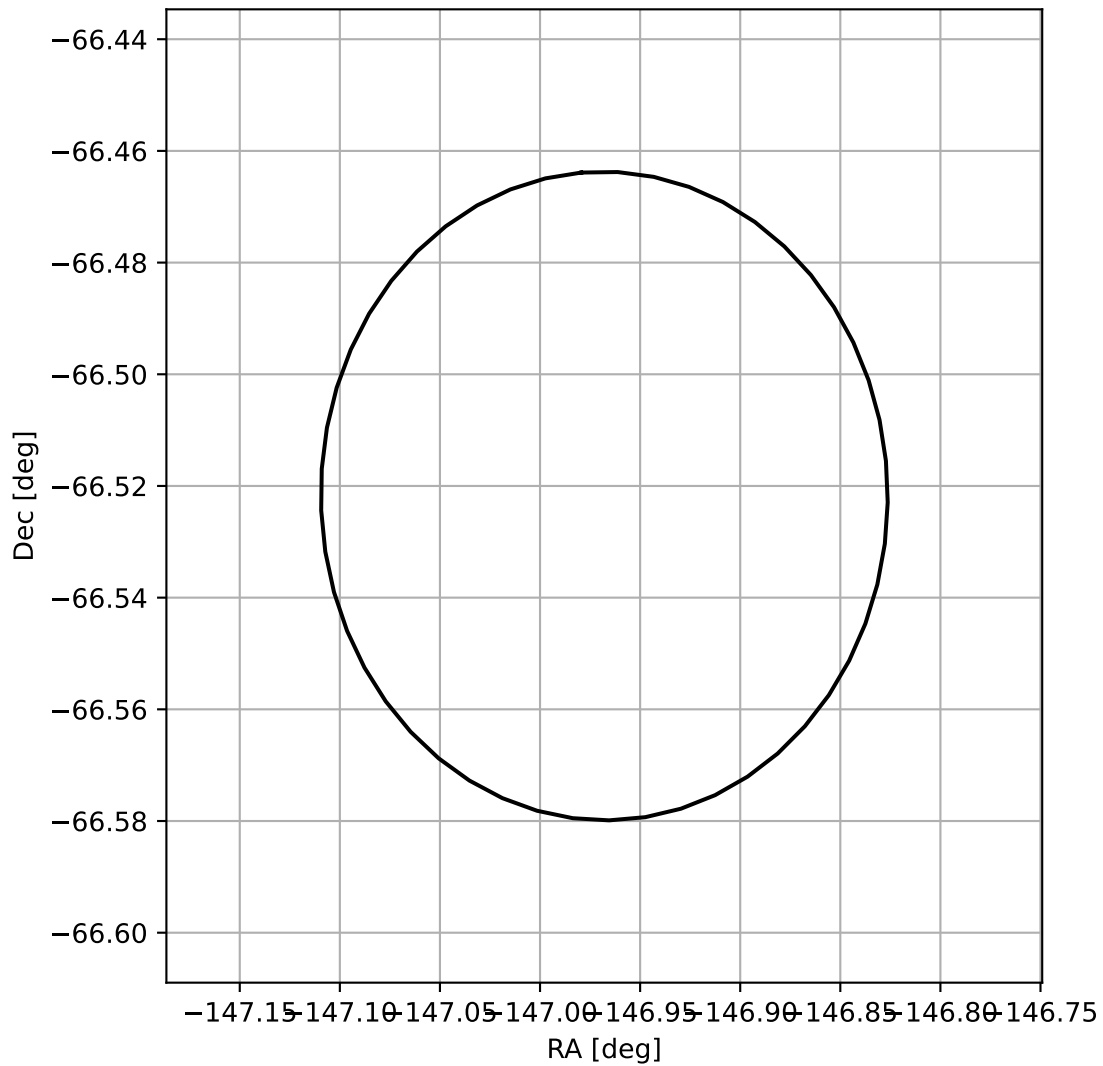
4FGL J1412.1-6631
