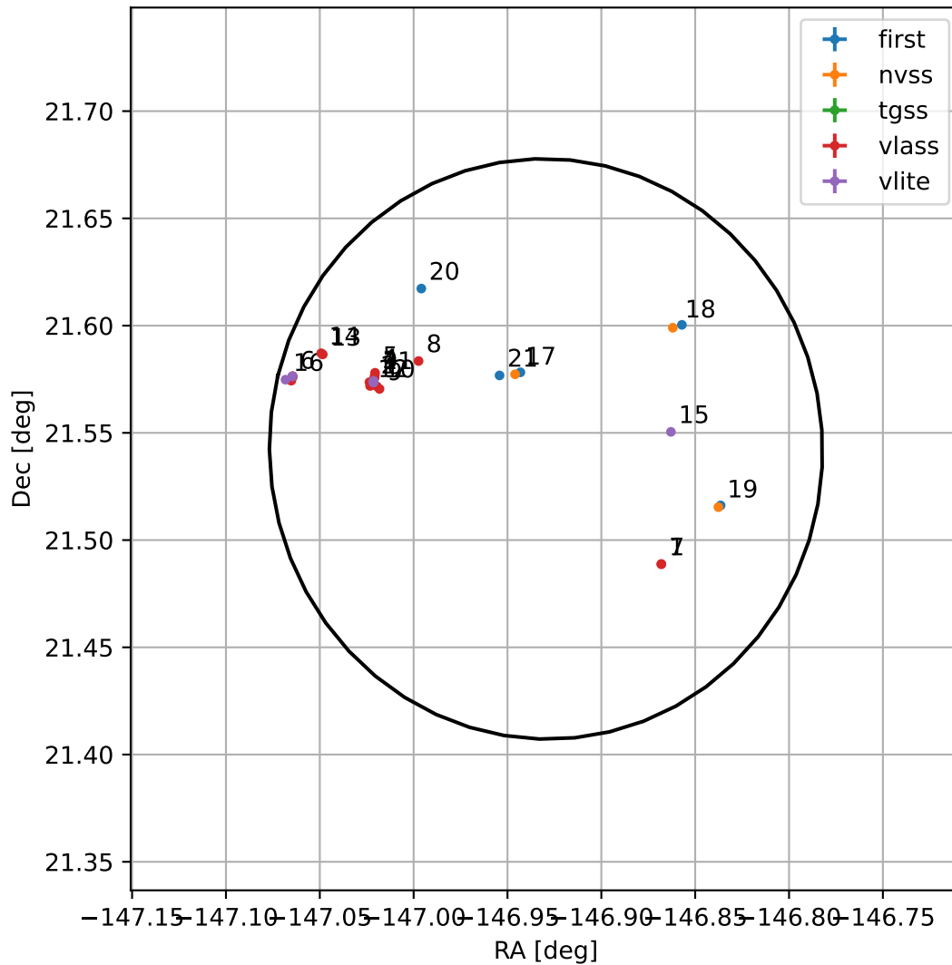
4FGL J1412.2+2132
