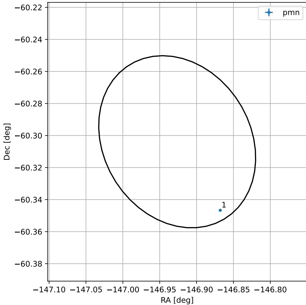
4FGL J1412.2-6018
