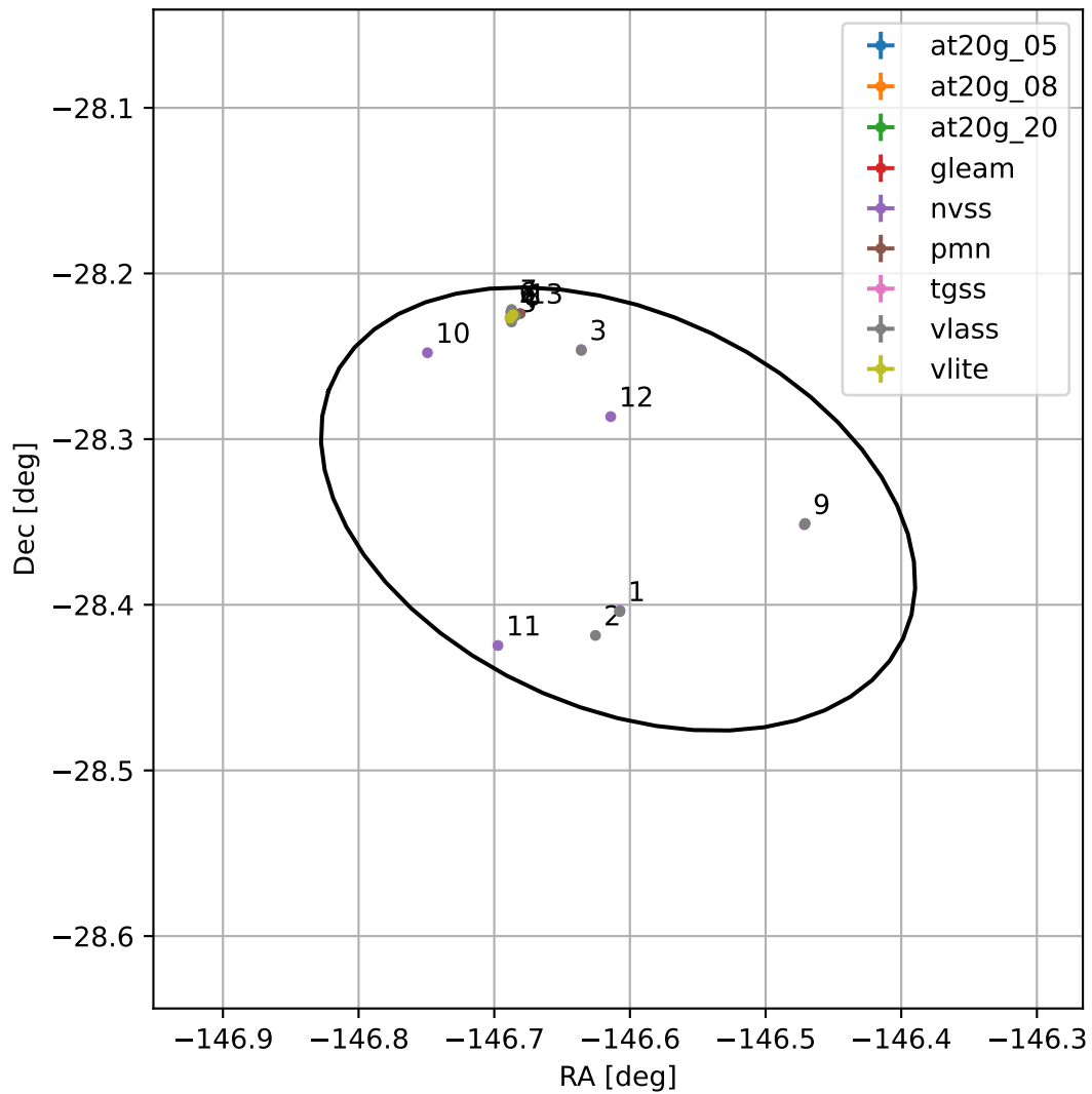
4FGL J1413.5-2820
