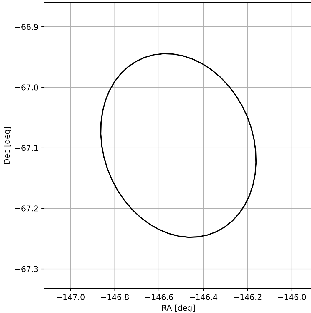
4FGL J1413.9-6705
