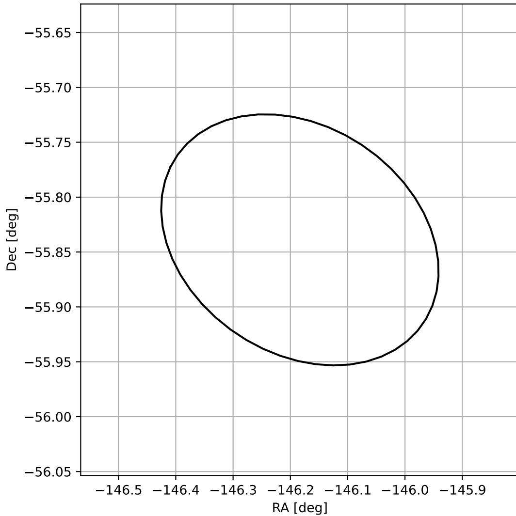
4FGL J1415.2-5550
