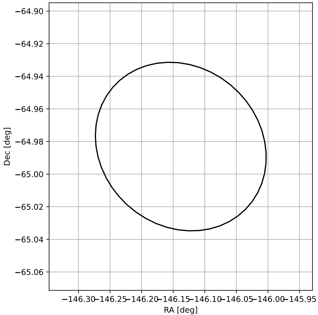
4FGL J1415.4-6458
