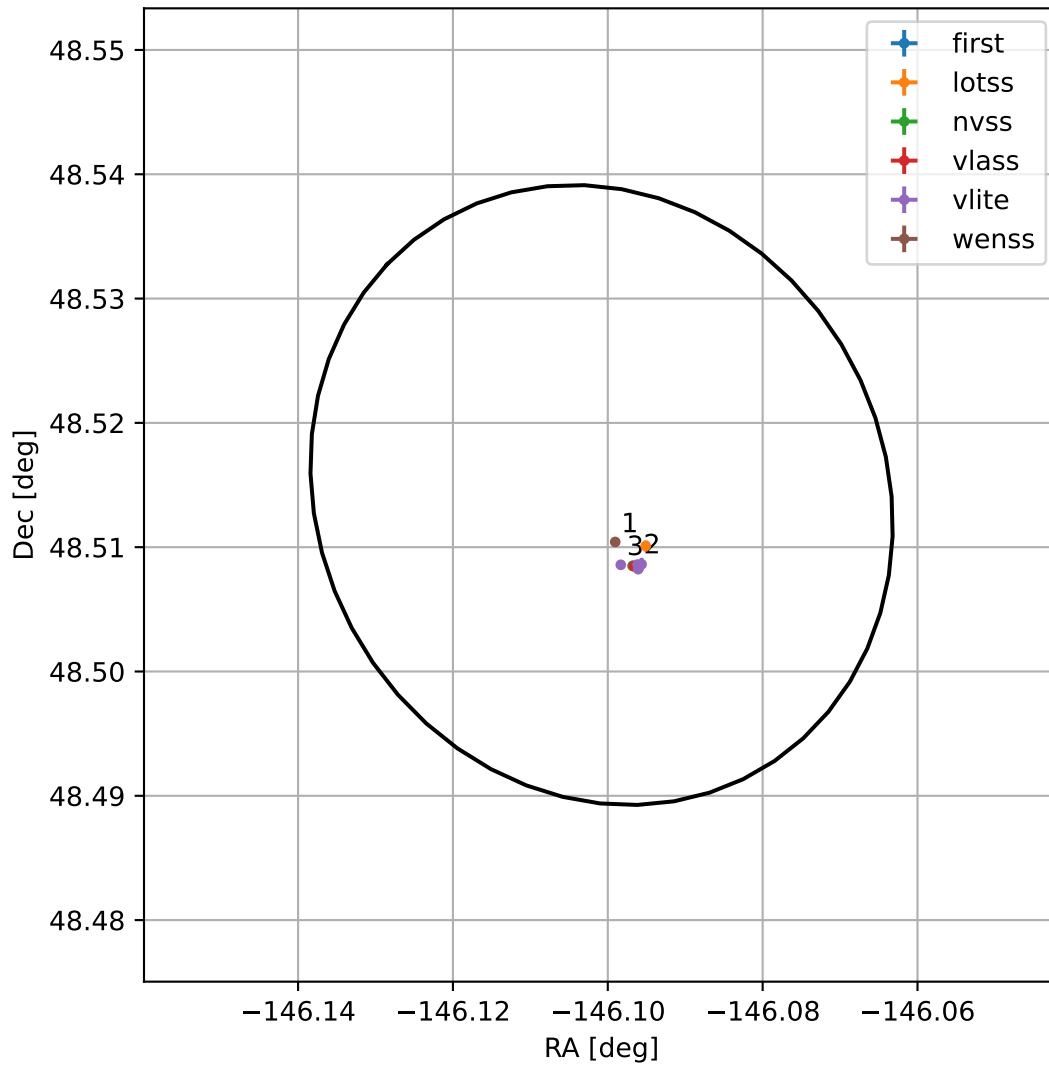
4FGL J1415.5+4830
