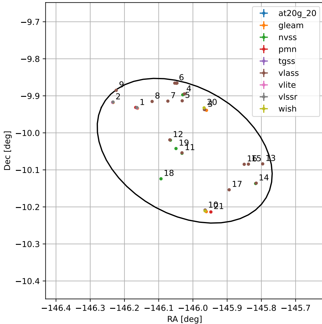
4FGL J1415.9-1002
