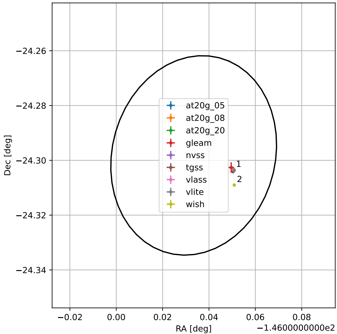
4FGL J1416.1-2417
