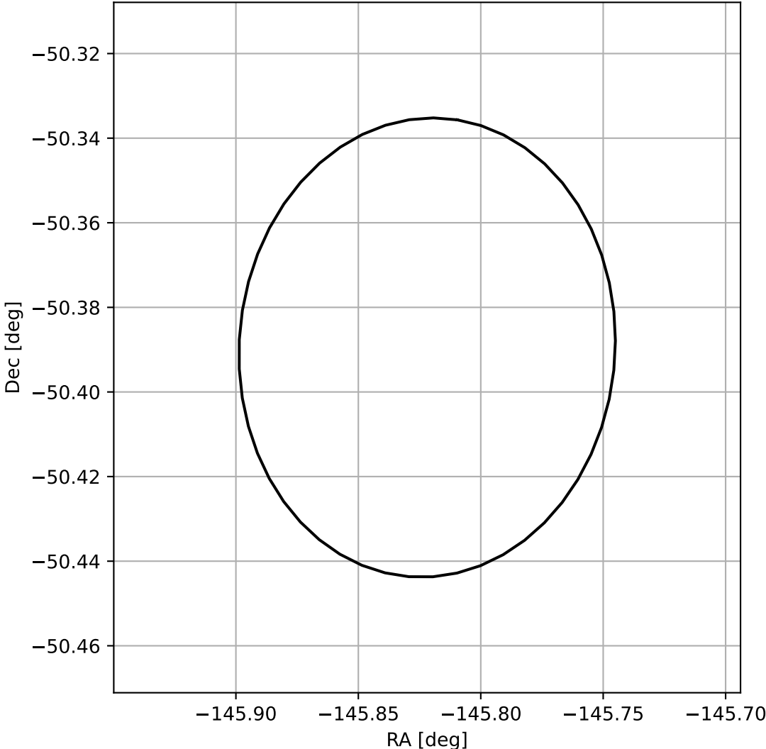
4FGL J1416.7-5023
