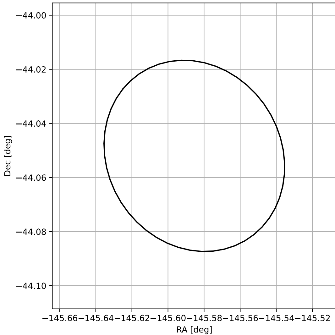
4FGL J1417.6-4403
