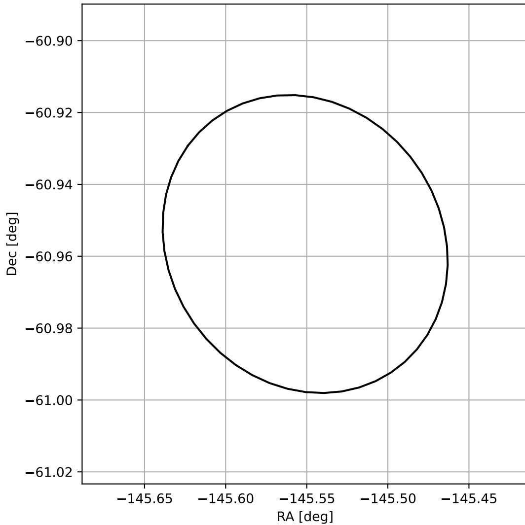
4FGL J1417.7-6057
