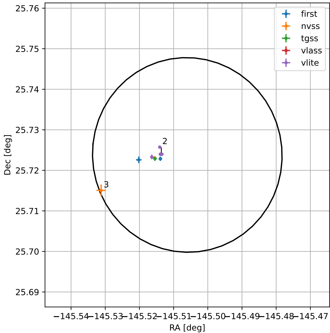
4FGL J1417.9+2543
