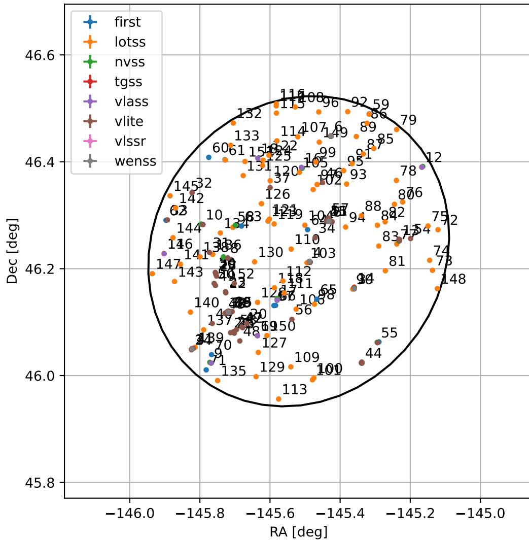
4FGL J1417.9+4613
