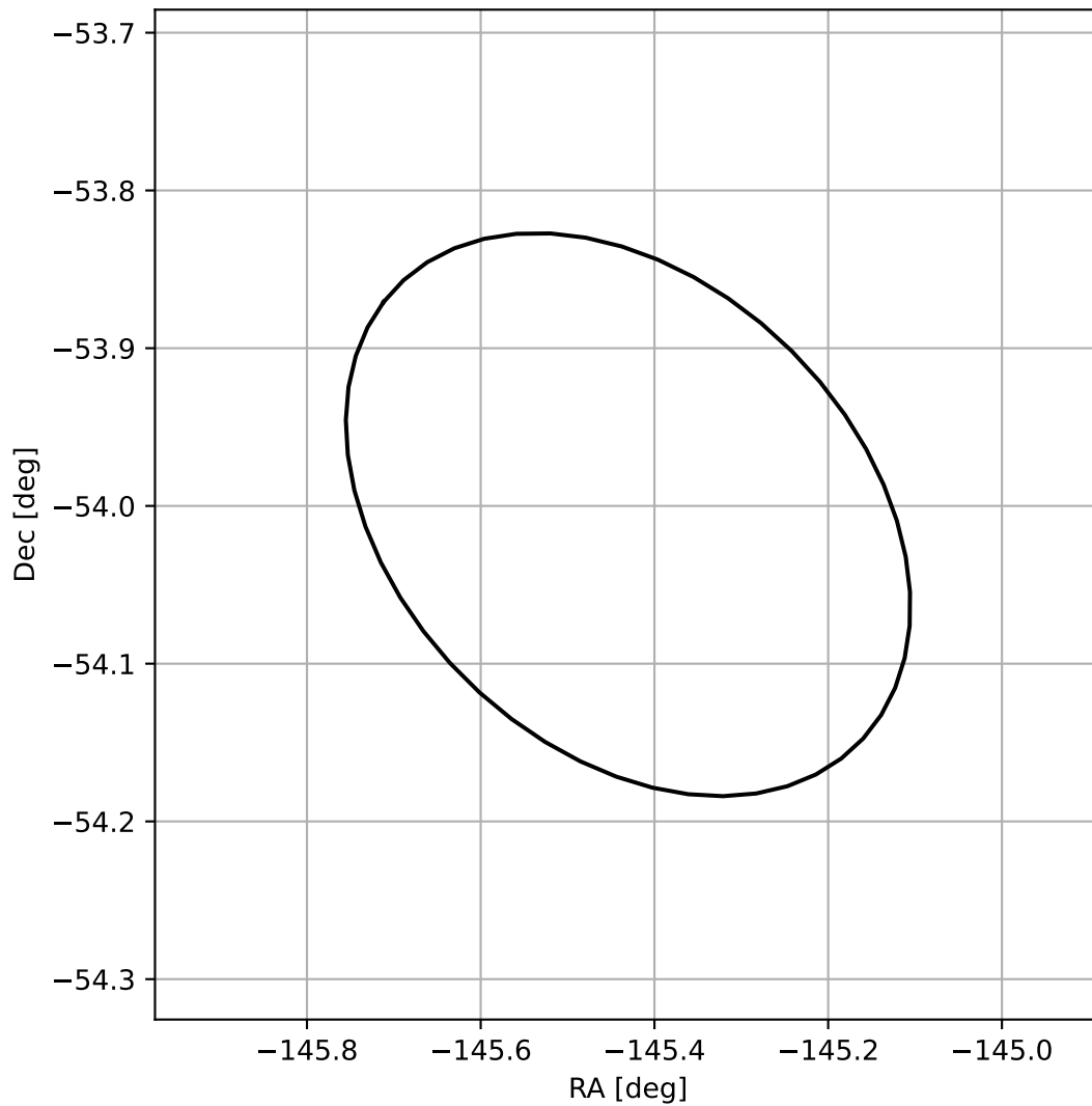
4FGL J1418.2-5400
