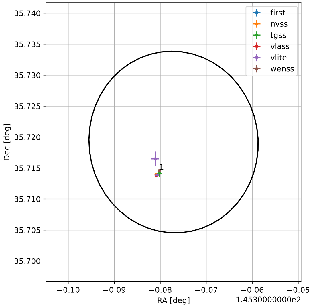
4FGL J1418.4+3543
