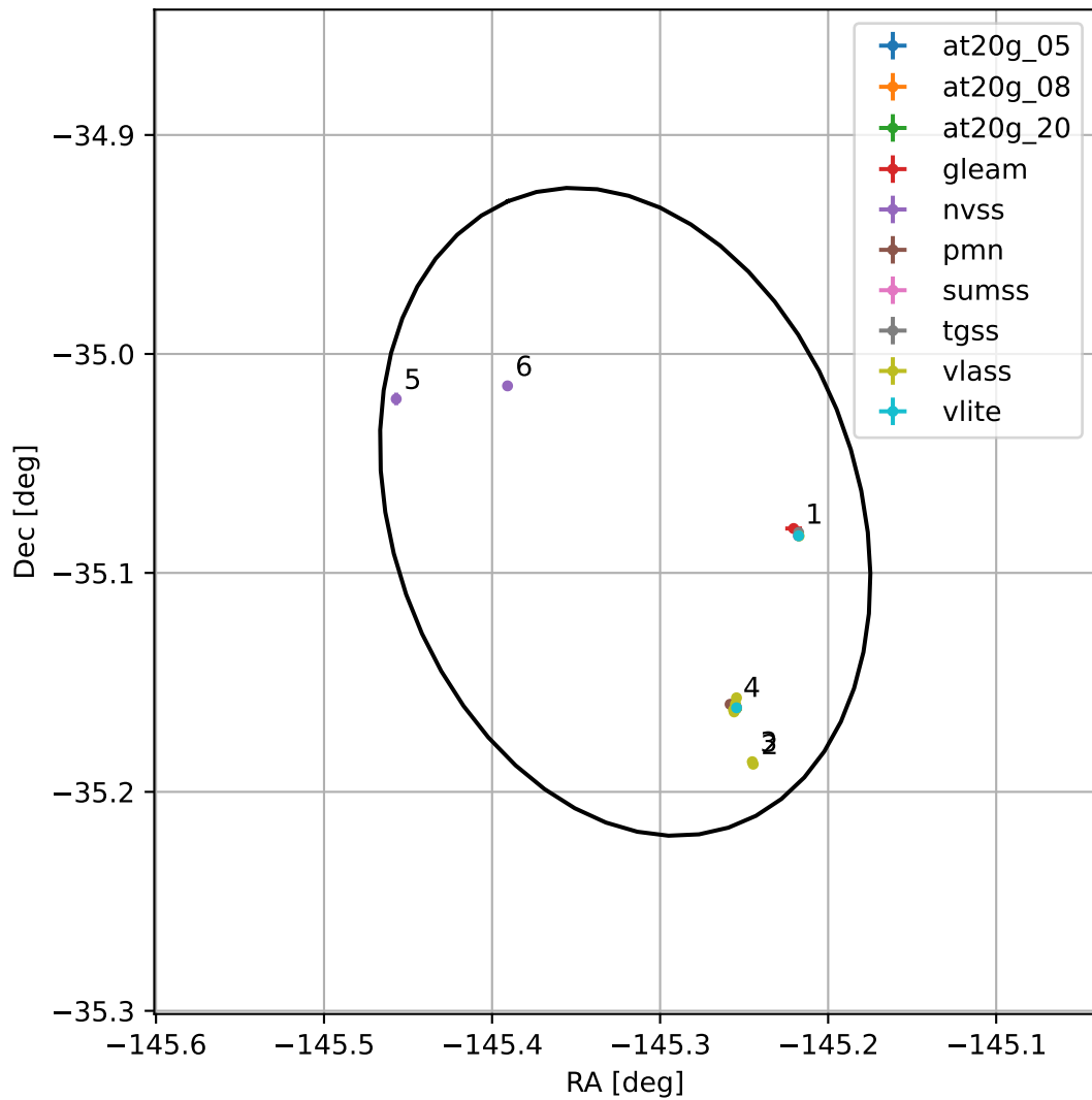
4FGL J1418.7-3504
