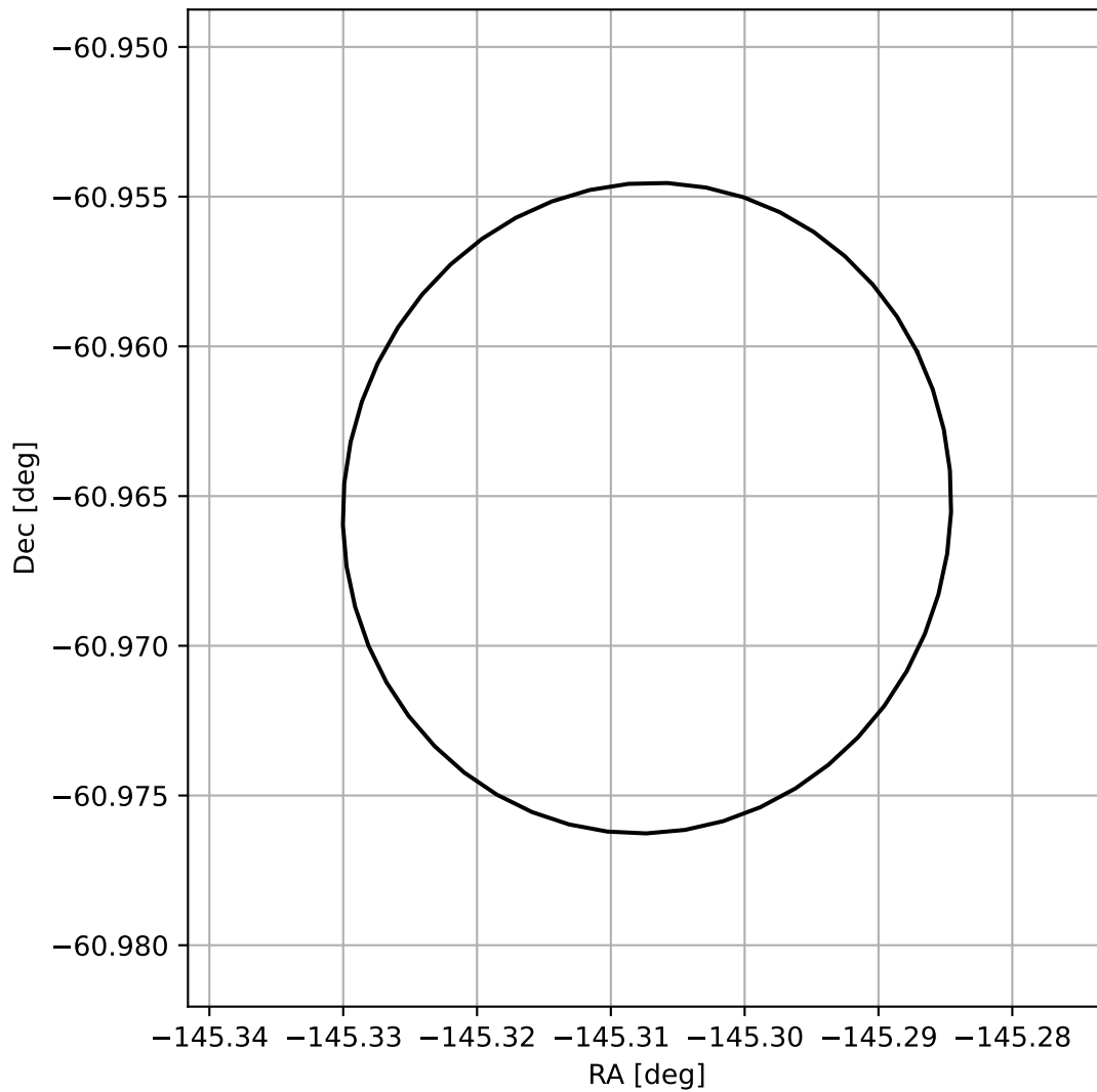
4FGL J1418.7-6057
