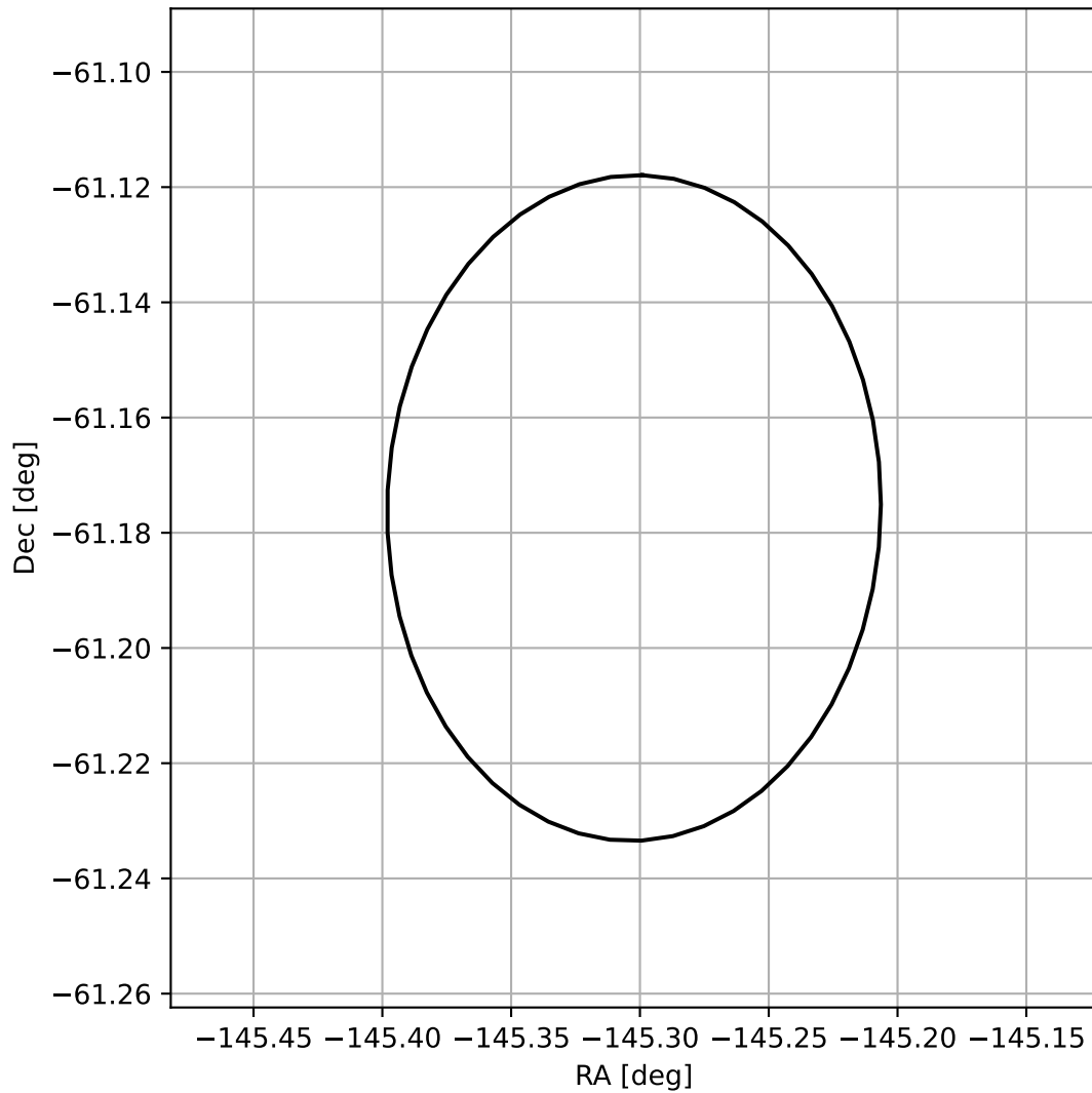
4FGL J1418.7-6110
