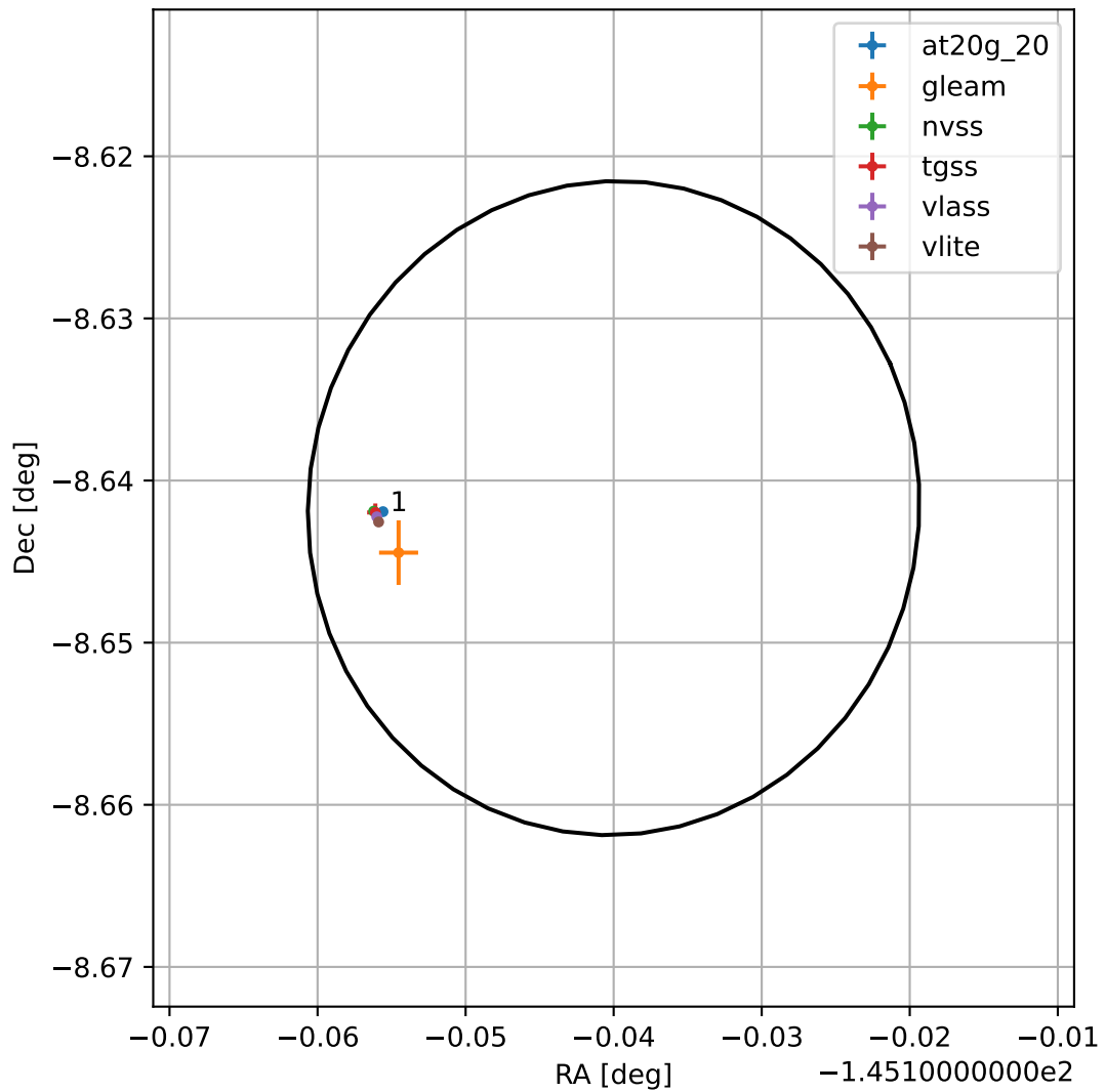
4FGL J1419.4-0838
