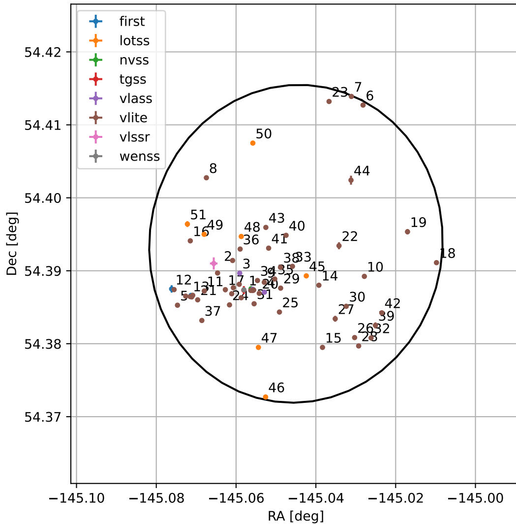
4FGL J1419.8+5423
