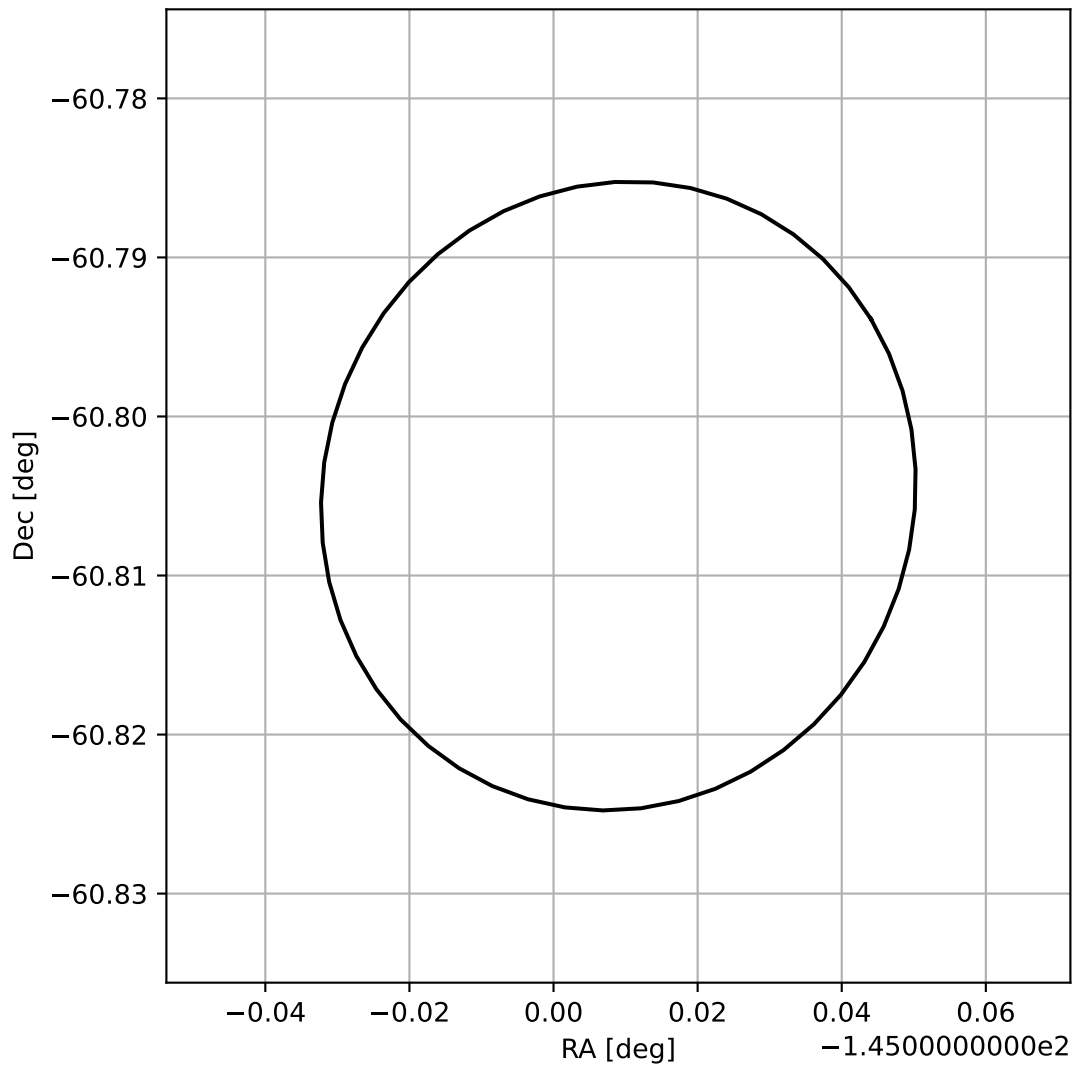
4FGL J1420.0-6048
