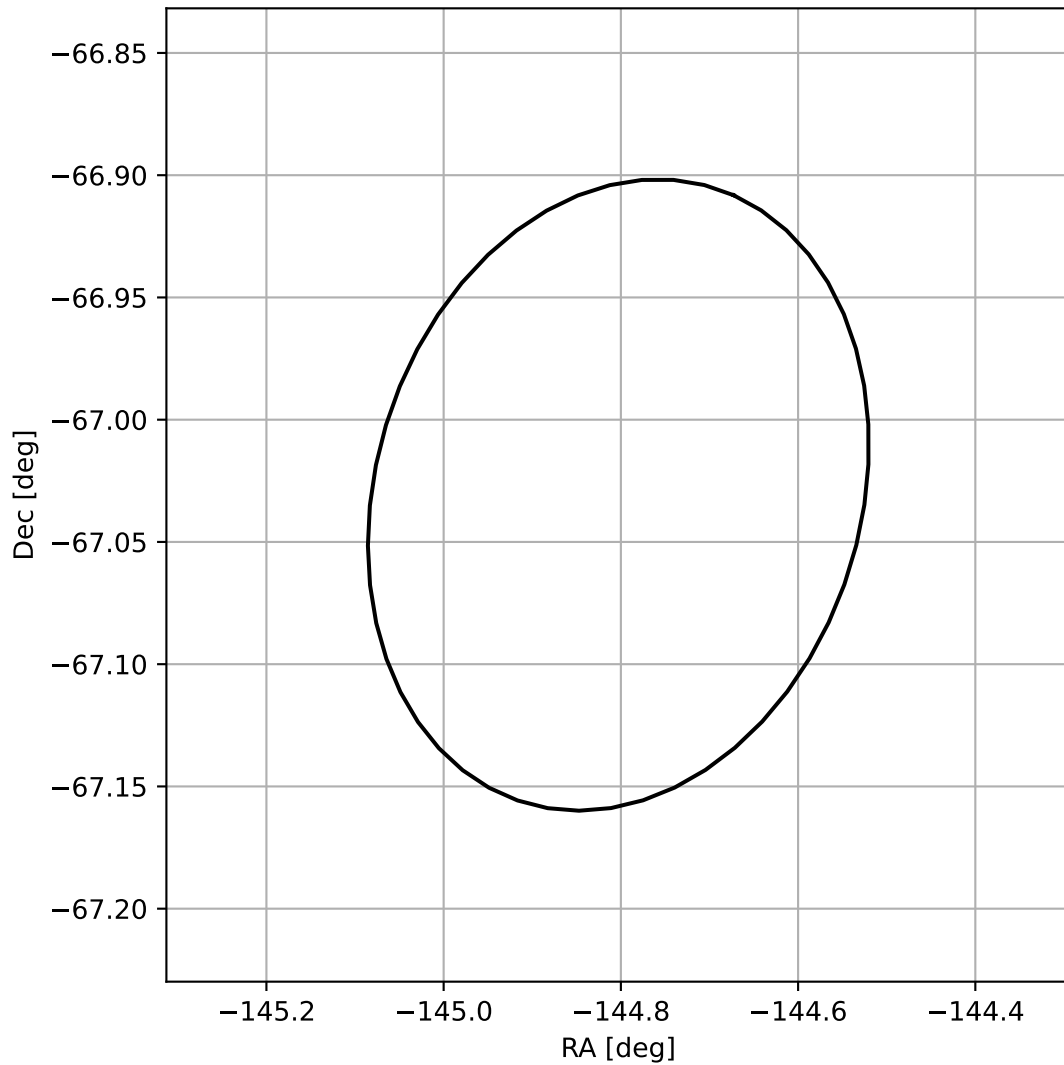
4FGL J1420.7-6701
