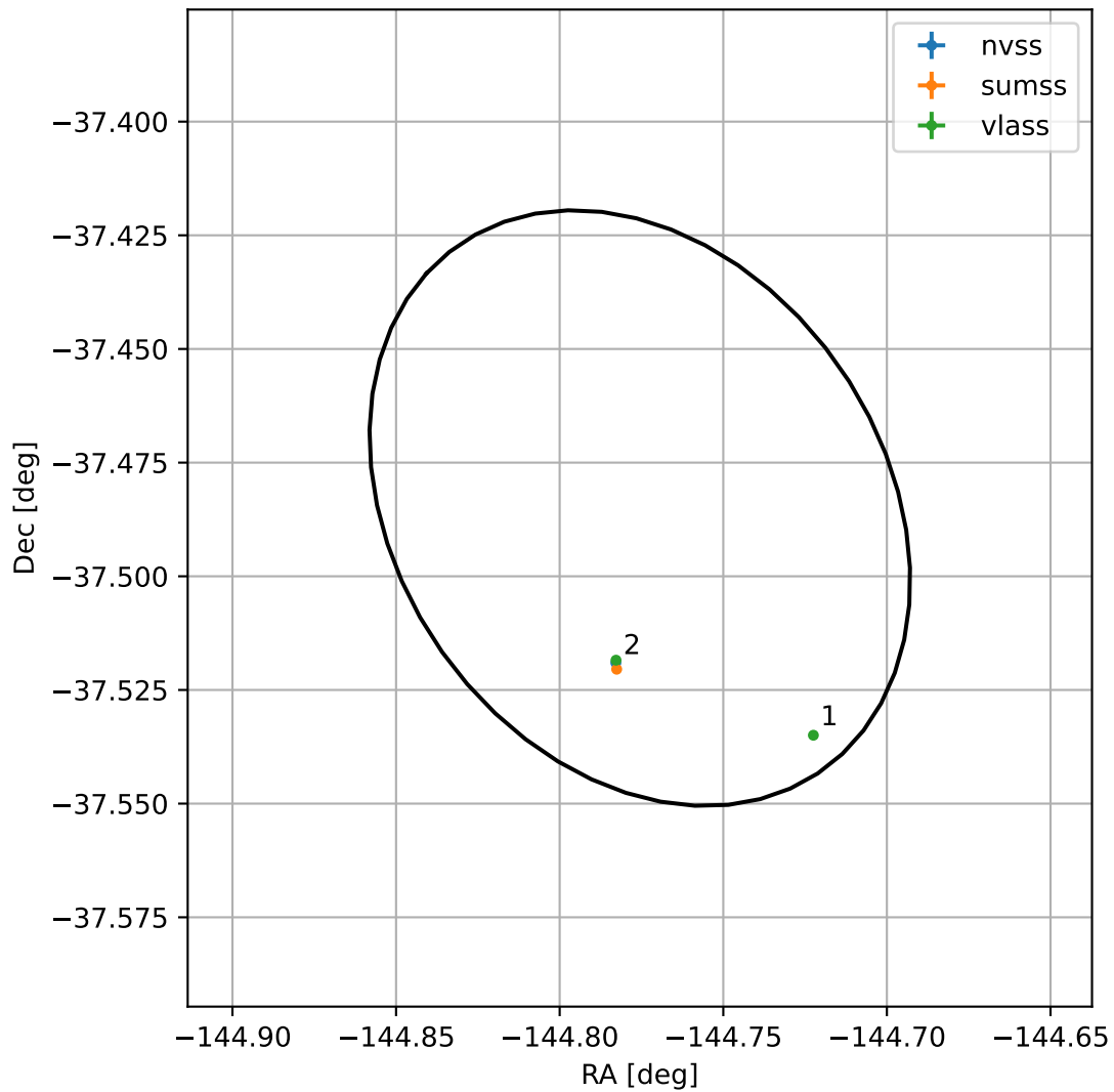
4FGL J1420.8-3729
