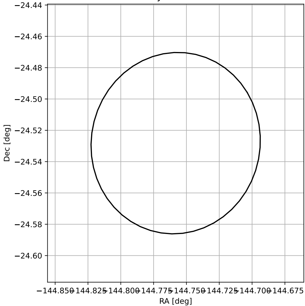
4FGL J1420.9-2431
