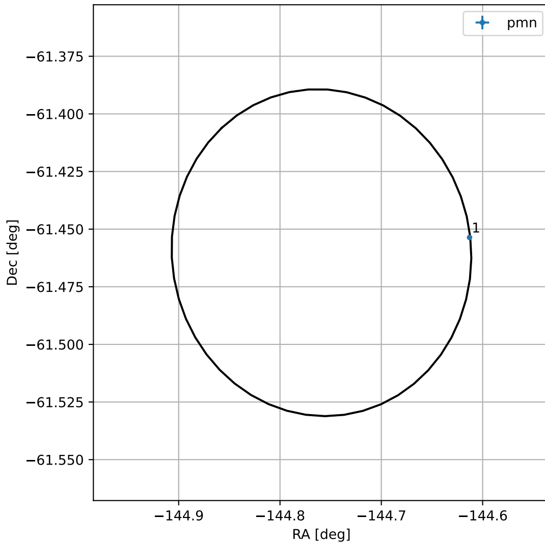
4FGL J1420.9-6127
