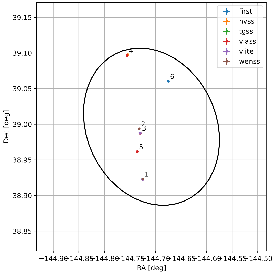
4FGL J1421.1+3859
