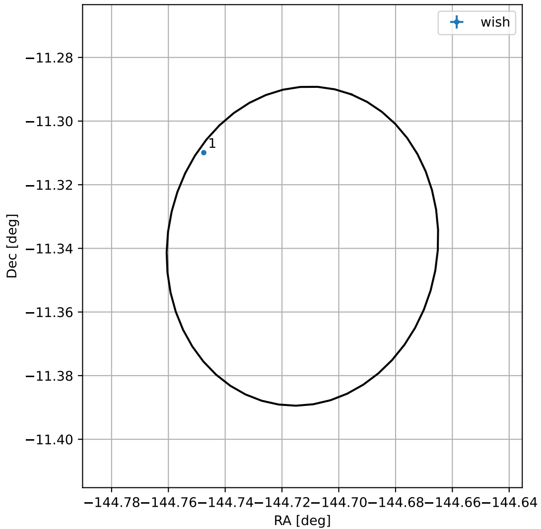
4FGL J1421.1-1120
