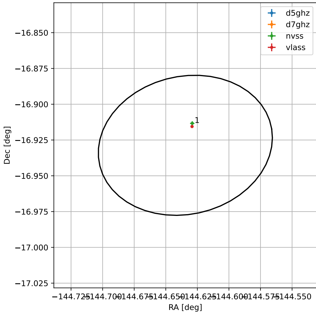
4FGL J1421.4-1655
