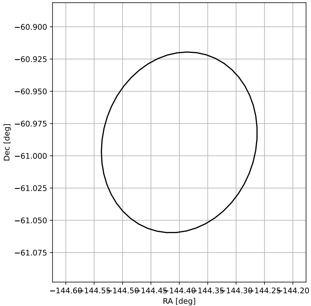
4FGL J1422.3-6059
