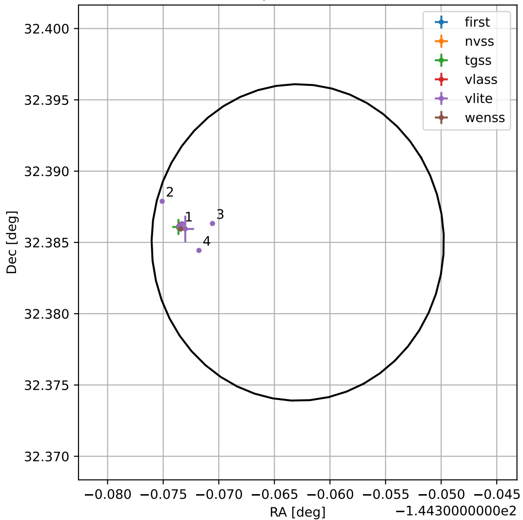
4FGL J1422.5+3223
