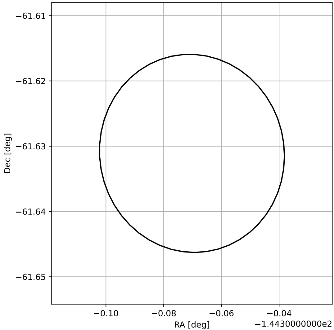
4FGL J1422.5-6137
