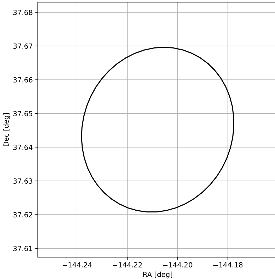
4FGL J1423.1+3738
