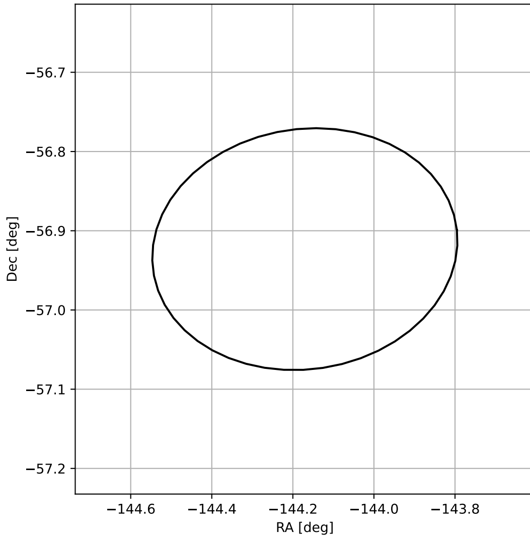
4FGL J1423.3-5655
