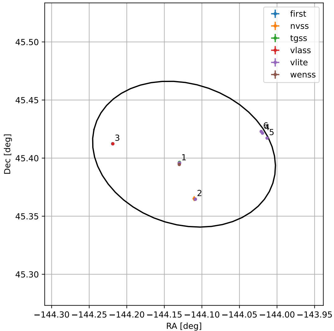
4FGL J1423.5+4524
