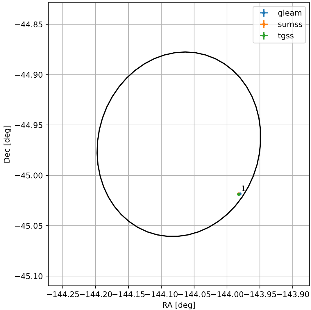
4FGL J1423.7-4458
