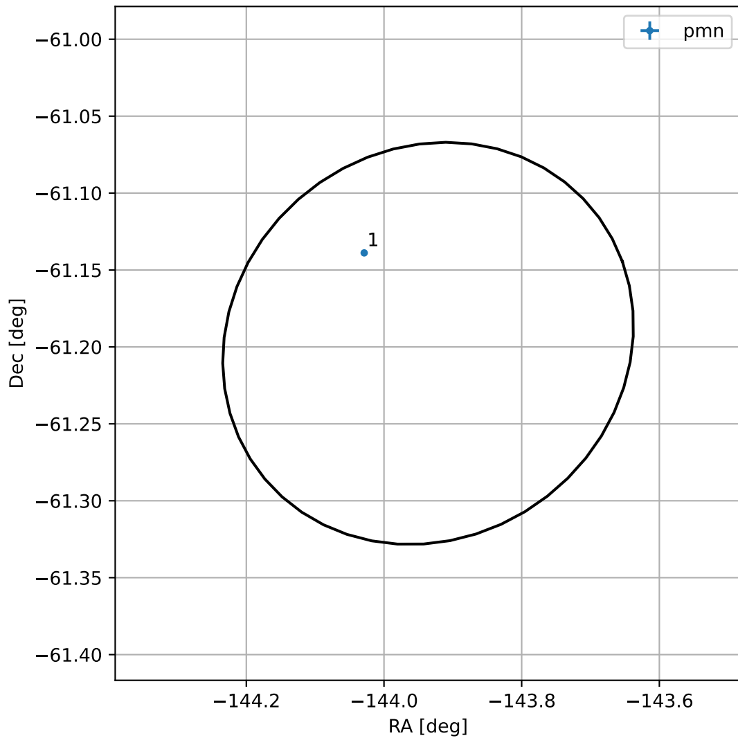
4FGL J1424.2-6111
