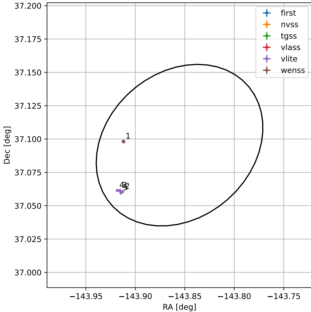
4FGL J1424.5+3705
