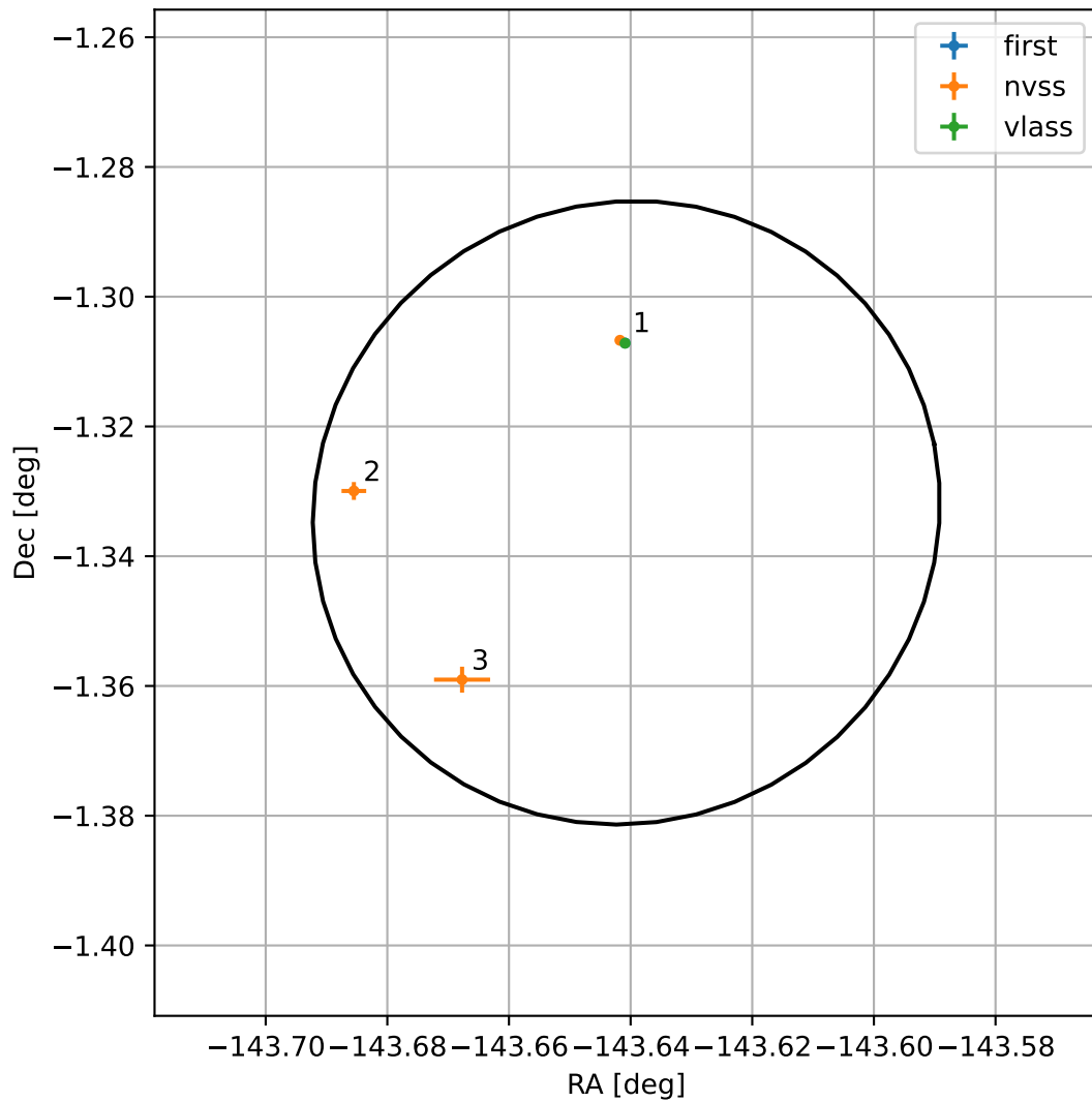
4FGL J1425.4-0119
