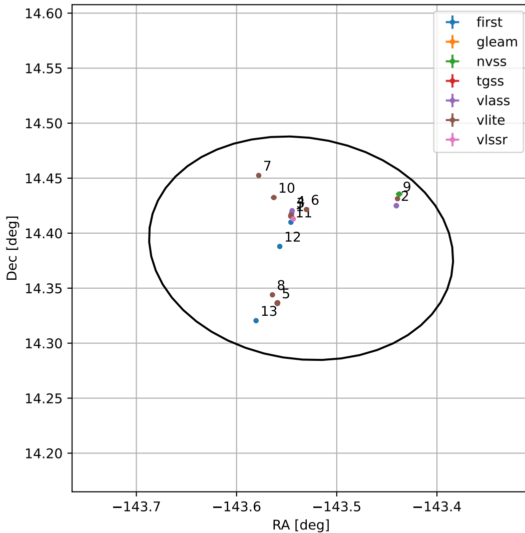
4FGL J1425.8+1423
