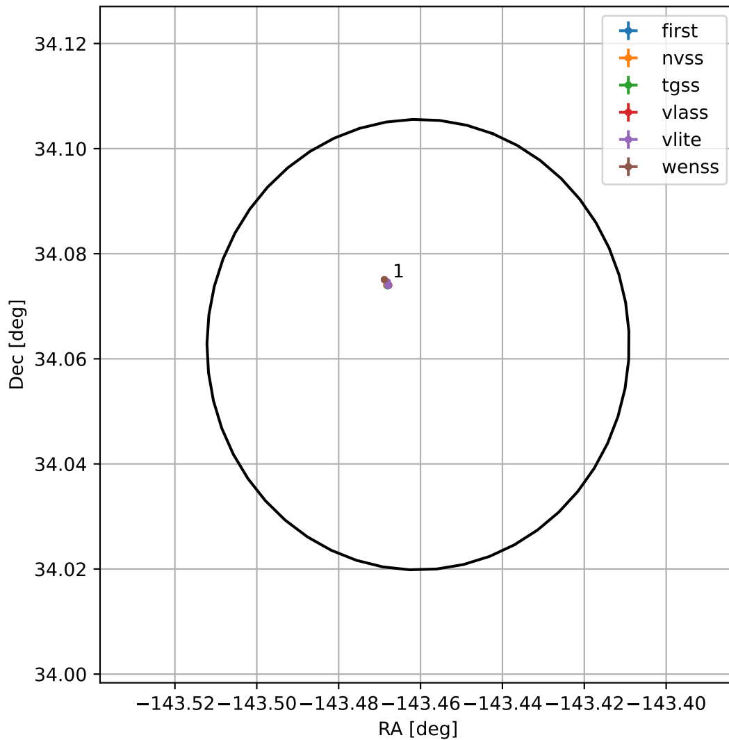
4FGL J1426.1+3403
