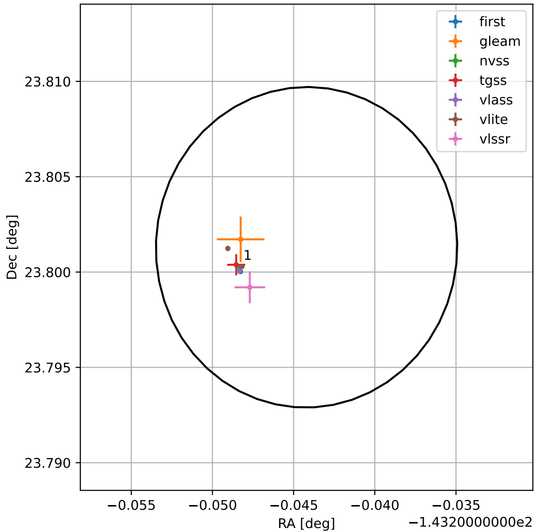
4FGL J1427.0+2348
