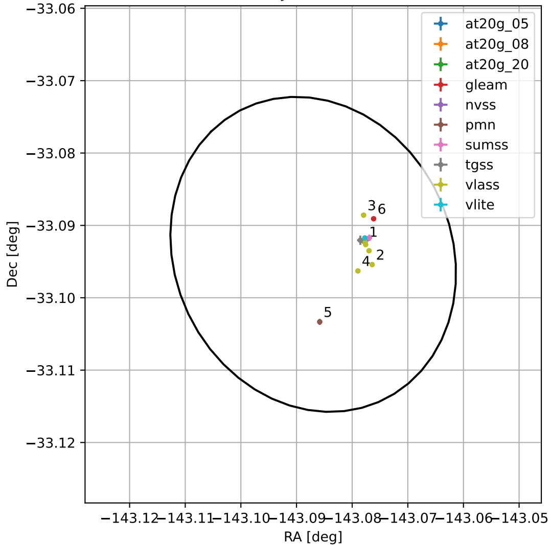
4FGL J1427.6-3305
