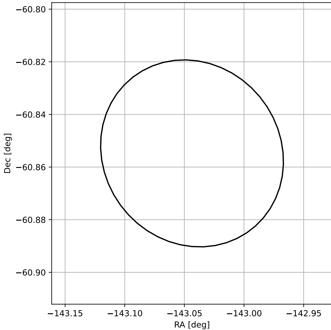
4FGL J1427.8-6051
