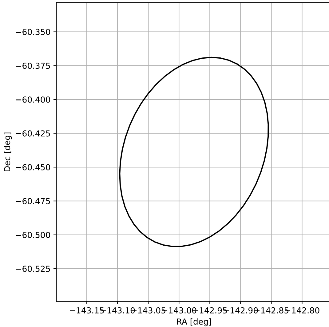
4FGL J1428.0-6026
